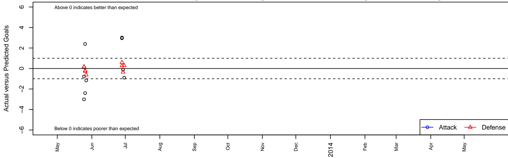
WAFC Storm G01 Dots are actual minus expected GF (blue circles) and GA (red triangles). Blue line is smoothed change in attack strength. Red is smoothed change in defense strength.
